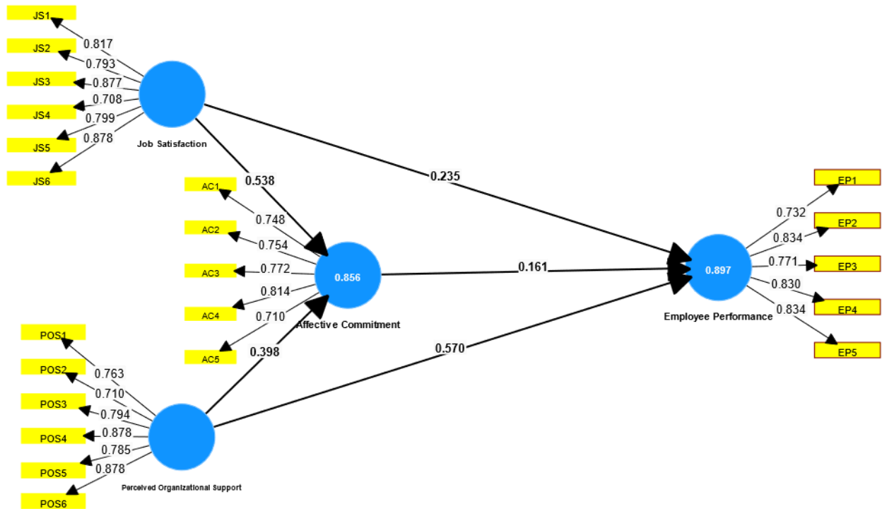
Fig.2: Path analysis
