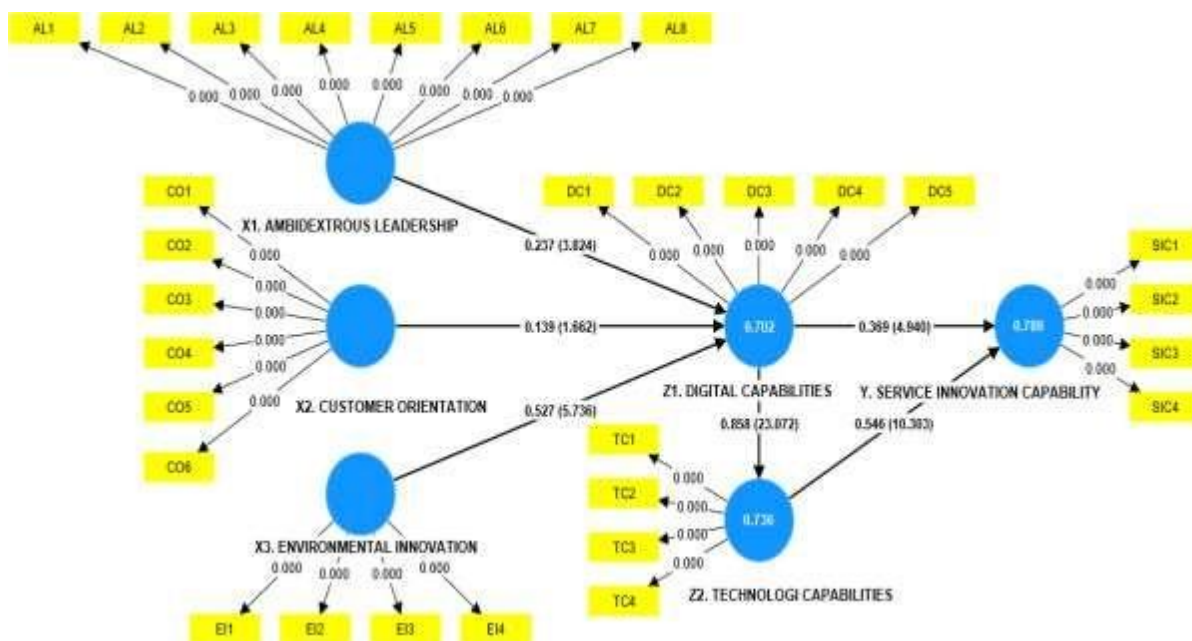
Fig.2: Display of PLS Algorithm Calculation Results
