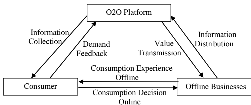
Figure 1: O2O Model
