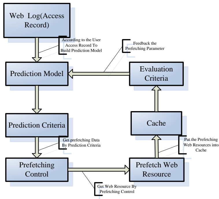
Fig 1 Prefetching Model
